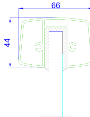
HRA64X44 RECTANGLE HANDRAIL
